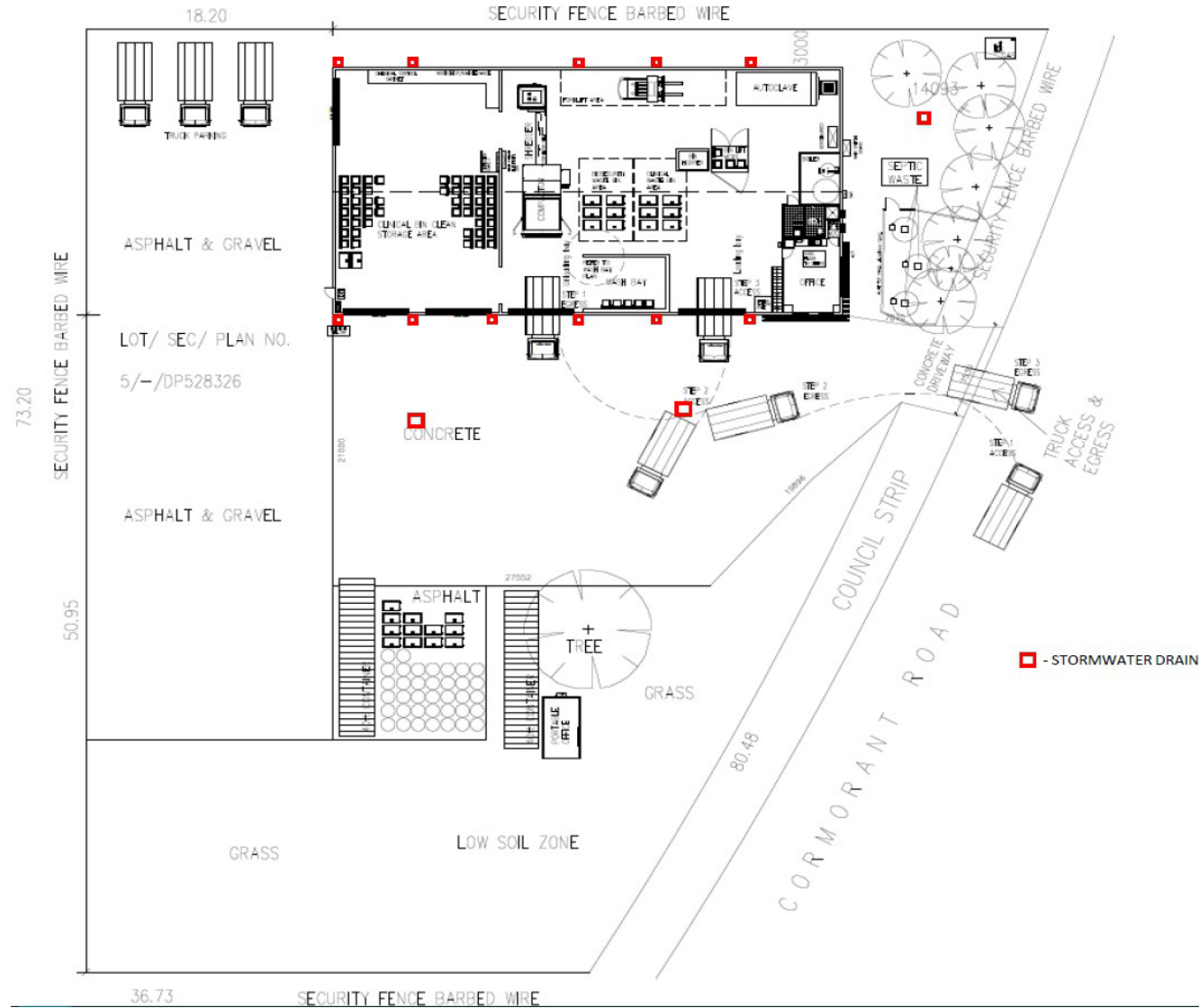
Figure 4 Med-X Facility Newcastle Site Plan
