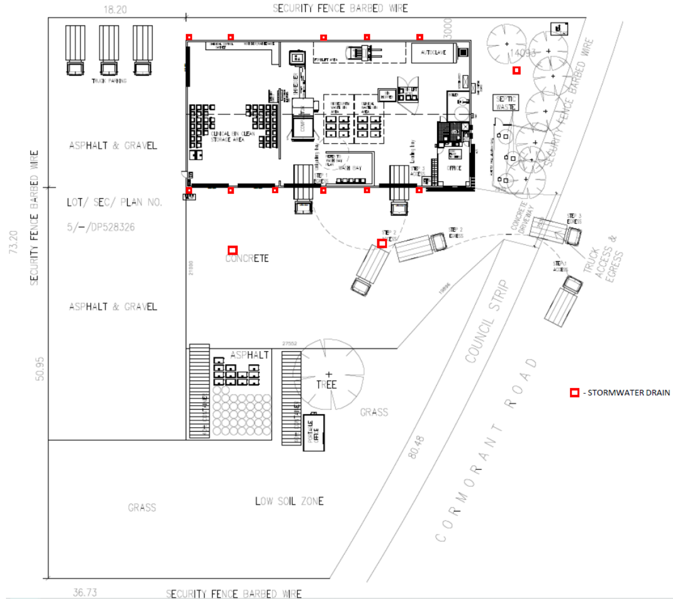
Figure 4 Med-X Facility Newcastle Site Plan Uncontrolled when printed
