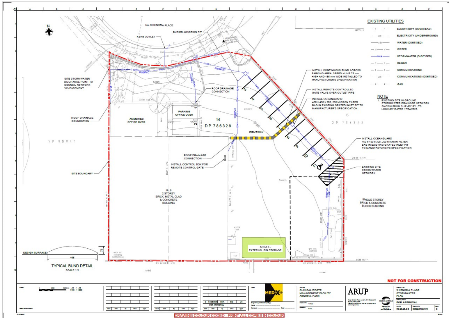
Figure 3 Med-X Facility Arndell Park Site Plan
